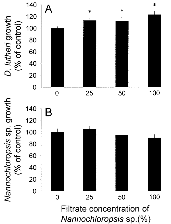
Fig. 4. Effects of various concentrations of Nannochloropsis sp. filtrates on the growth of D. lutheri (A) and Nannochloropsis sp. (B). Data are means \pm SD (% of control growth) of triplicate measurements. The asterisk (*) indicates a significant difference at P < 0.05 between the control and the experimental groups.
