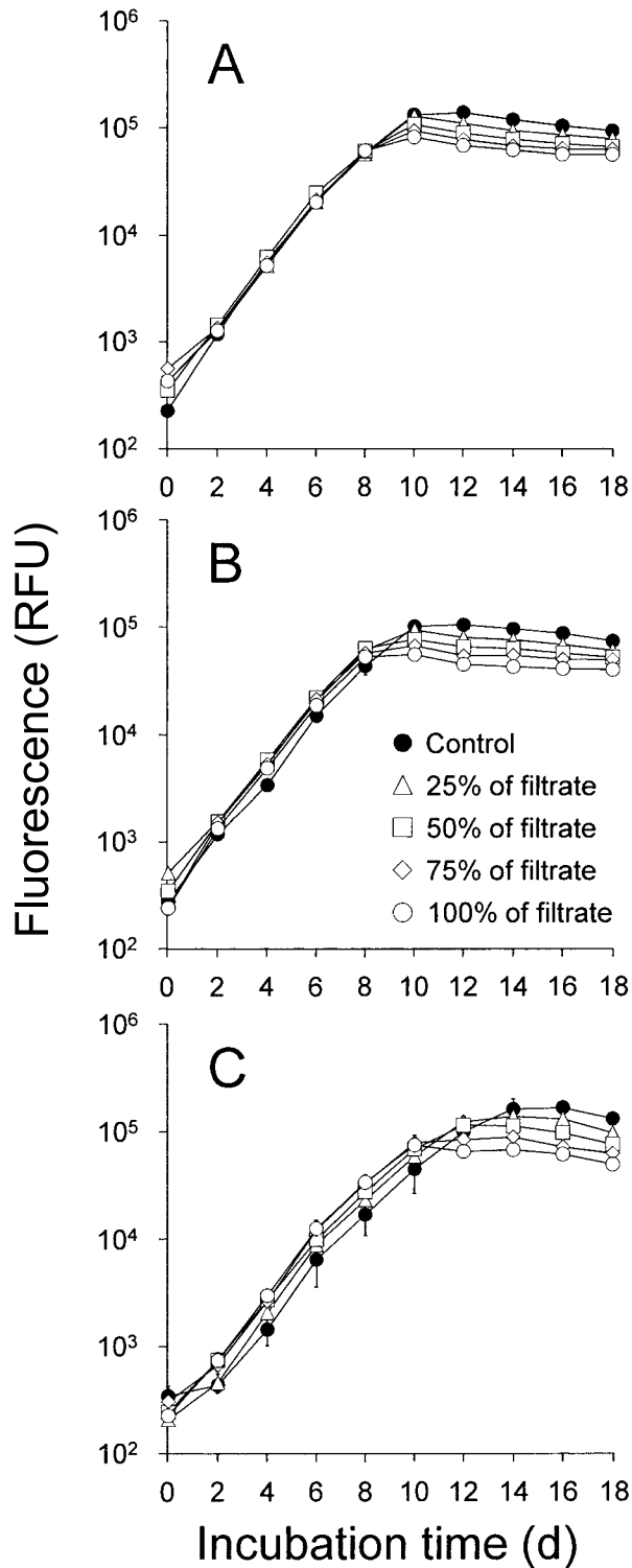
Fig. 3. Growth curves at 25°C of D. lutheri cells exposed to various concentrations of D. lutheri filtrates. A: cultivation temperature for preparation of D. lutheri filtrates was 15°C, B: cultivation temperature for preparation of D. lutheri filtrates was 20°C, and C: cultivation temperature for preparation of D. lutheri filtrates was 25°C. Data are means \pm SD (RFU) of triplicate measurements.
