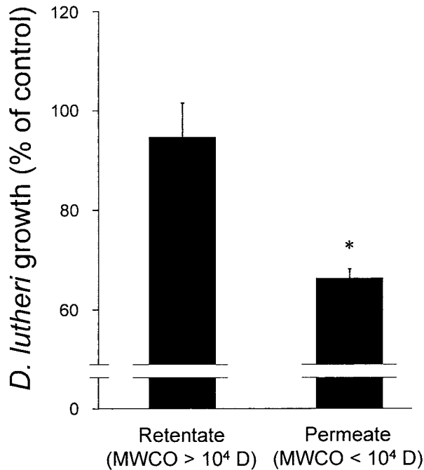
Fig. 5. Effects on the growth of D. lutheri of retentate (MWCO > 10 kDa) and permeate (MWCO < 10 kDa) fractions obtained by ultrafiltration of D. lutheri filtrates. Data are means \pm SD (% of control growth) of triplicate measurements. The asterisk (*) indicates a significant difference at P < 0.05 between the control and the experimental groups.
