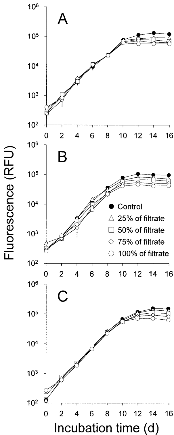
Fig. 1. Growth curves at 15°C of D. lutheri cells exposed to various concentrations of D. lutheri filtrates. A: cultivation temperature for preparation of D. lutheri filtrates was 15°C, B: cultivation temperature for preparation of D. lutheri filtrates was 20°C, and C: cultivation temperature for preparation of D. lutheri filtrates was 25°C. Data are means \pm SD (relative fluorescence units: RFU) of triplicate measurements.
