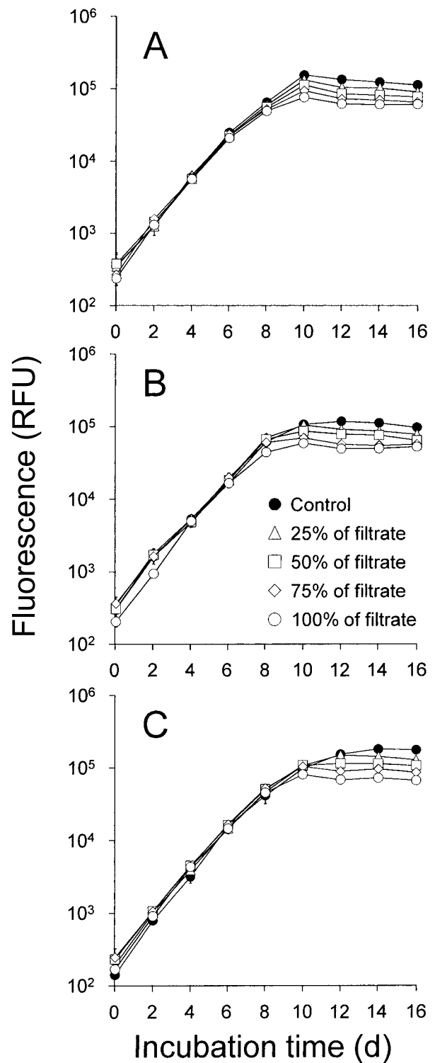
Fig. 2. Growth curves at 20°C of D. lutheri cells exposed to various concentrations of D. lutheri filtrates. A: cultivation temperature for preparation of D. lutheri filtrates was 15°C, B: cultivation temperature for preparation of D. lutheri filtrates was 20°C, and C: cultivation temperature for preparation of D. lutheri filtrates was 25°C. Data are means \pm SD (RFU) of triplicate measurements.
