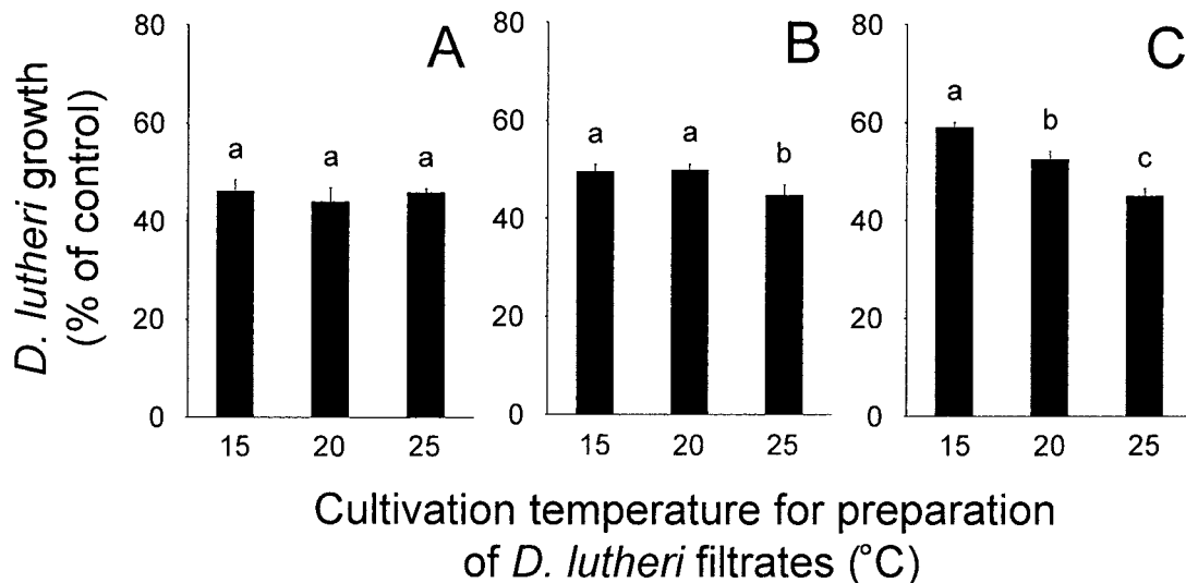
Fig. 6. Effects of D. lutheri filtrates on the growth of D. lutheri under various experimental sample preparation and growth conditions. A: temperature for growth experiments was 15°C, B: temperature for growth experiments was 20°C, and C: temperature for growth experiments was 25°C. Data are means \pm SD (% of control growth) of triplicate measurements. Values labeled with the same letters are not significantly different.
