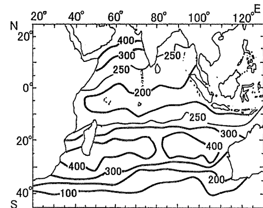
Fig. 8. Isothermal depth of 24^{\circ}\text{C} (upper) and 13^{\circ}\text{C} (lower)
