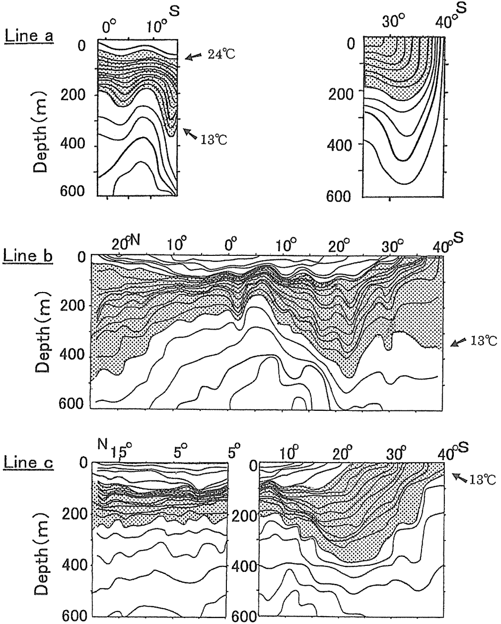
Fig. 9-1. Vertical profiles of average water temperatures in line a-c.
