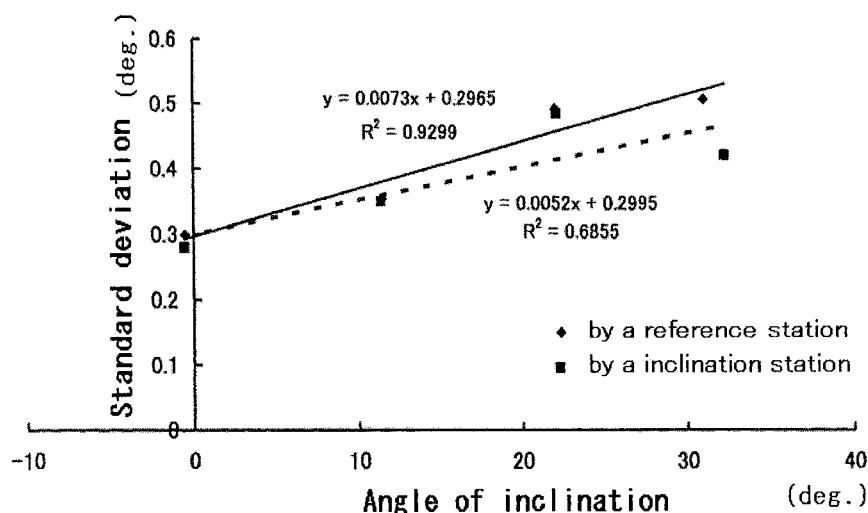
Fig. 6 . Measurement accuracy of the angle of inclination which was gained from the reference station and gained by making one side the inclined station.
