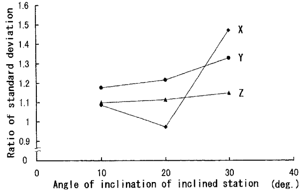
Fig. 4. Measurement accuracy by the inclined antenna.
