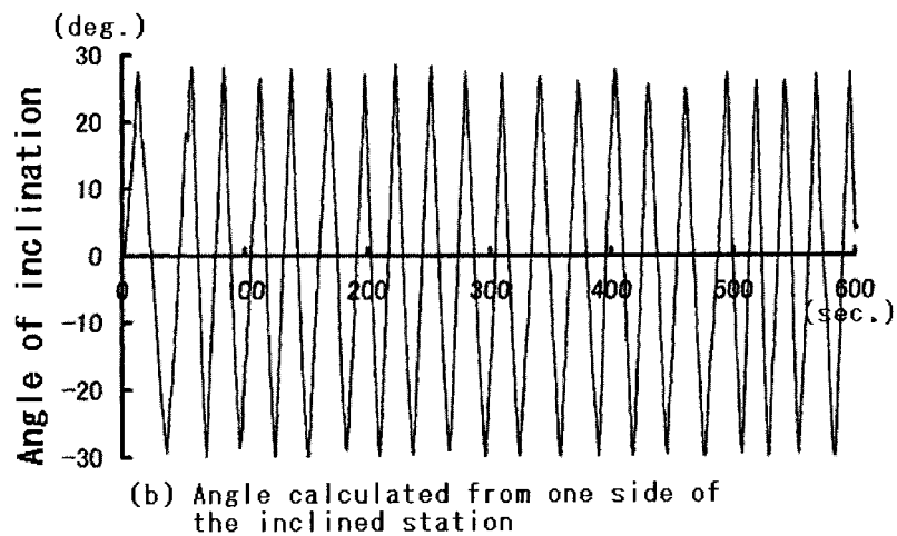
Fig. 8. An example of the result of the inclination experiment.
