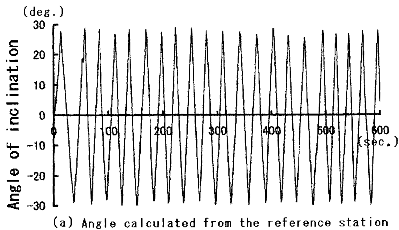
Fig. 7. An example of the measurement consequence to the z element at two inclined stations.
