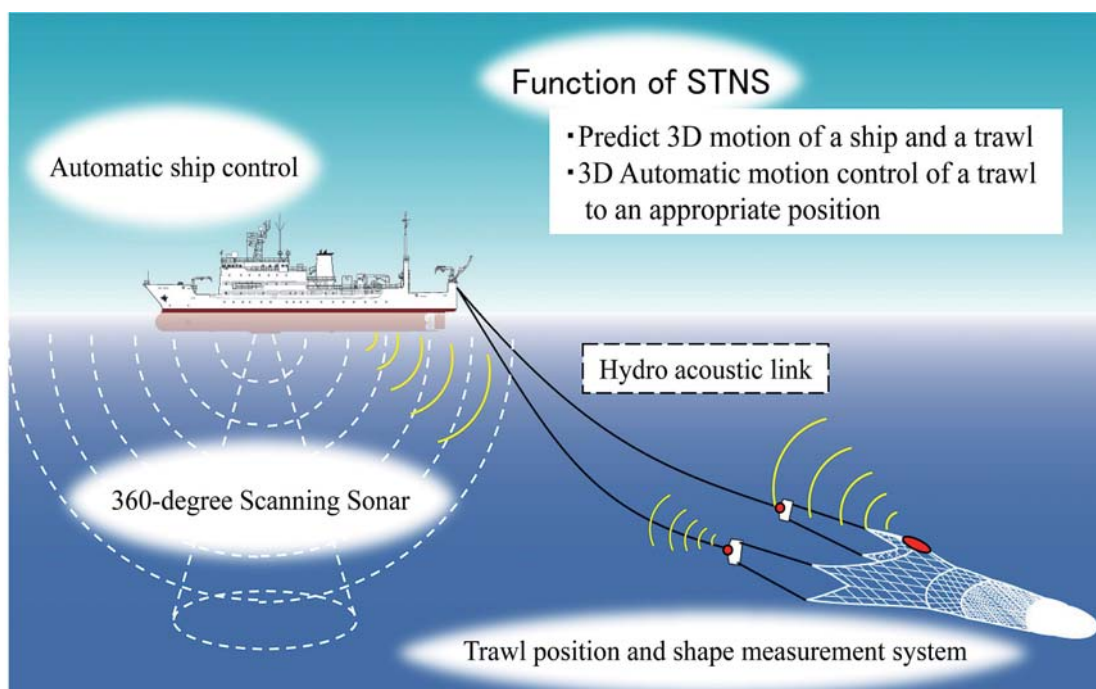
Fig. 1. The function of STN system.
