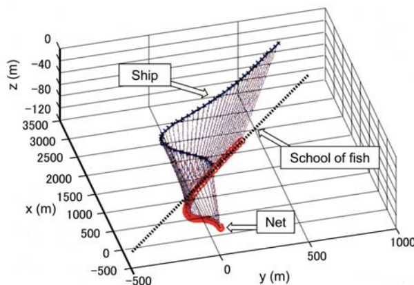
Fig. 6 . The simulation model of three-dimensional movement. (Mid-water trawl)
