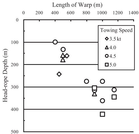
Fig. 8-1. The relationship between length of warp and the head rope depth in the experiments (Mid-water trawl).
