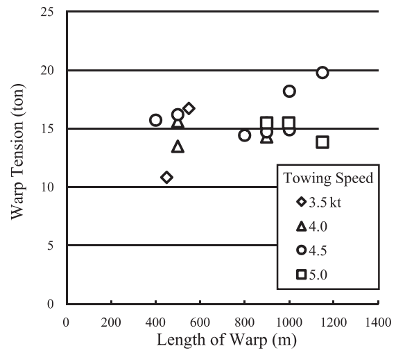
Fig. 8-6. The relationship between length of warp and warp tension in the experiments (Mid-water trawl).
